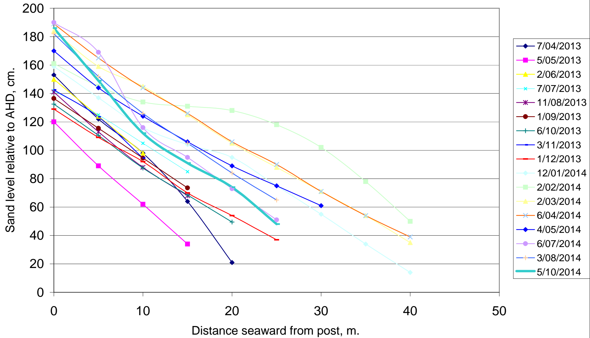
Post 8, Transverse Beach Profile
