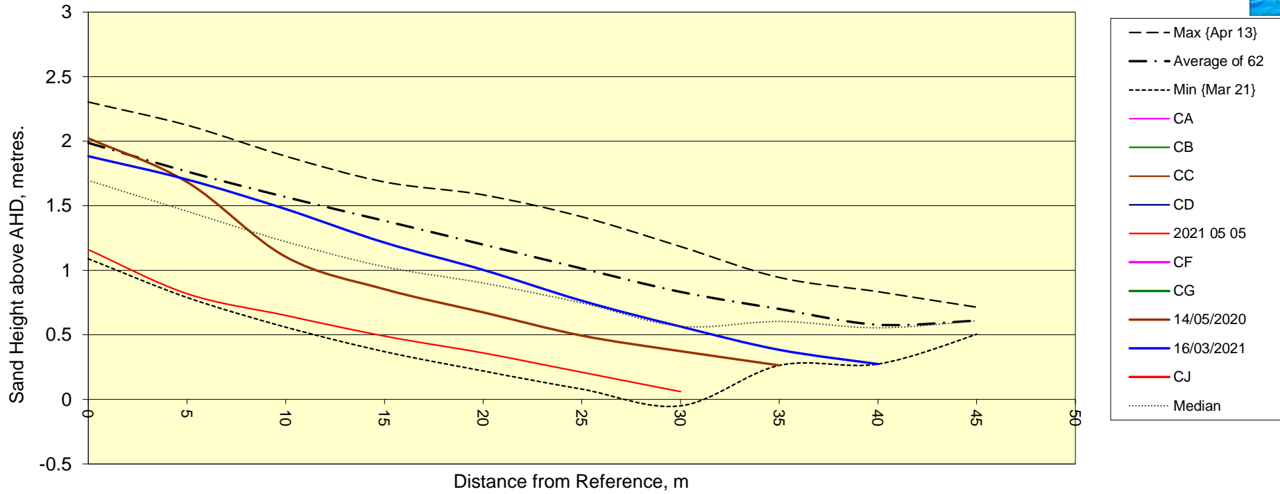
Chart PFEHTP1 Post 1 Transverse Profile perpendicular to dune scarp. (Legend date formats: dd/mm/yyyy = laser, yyyy mm dd = Propeller Aero, dd mmmyy = GPS) {Stats date range in braces}
