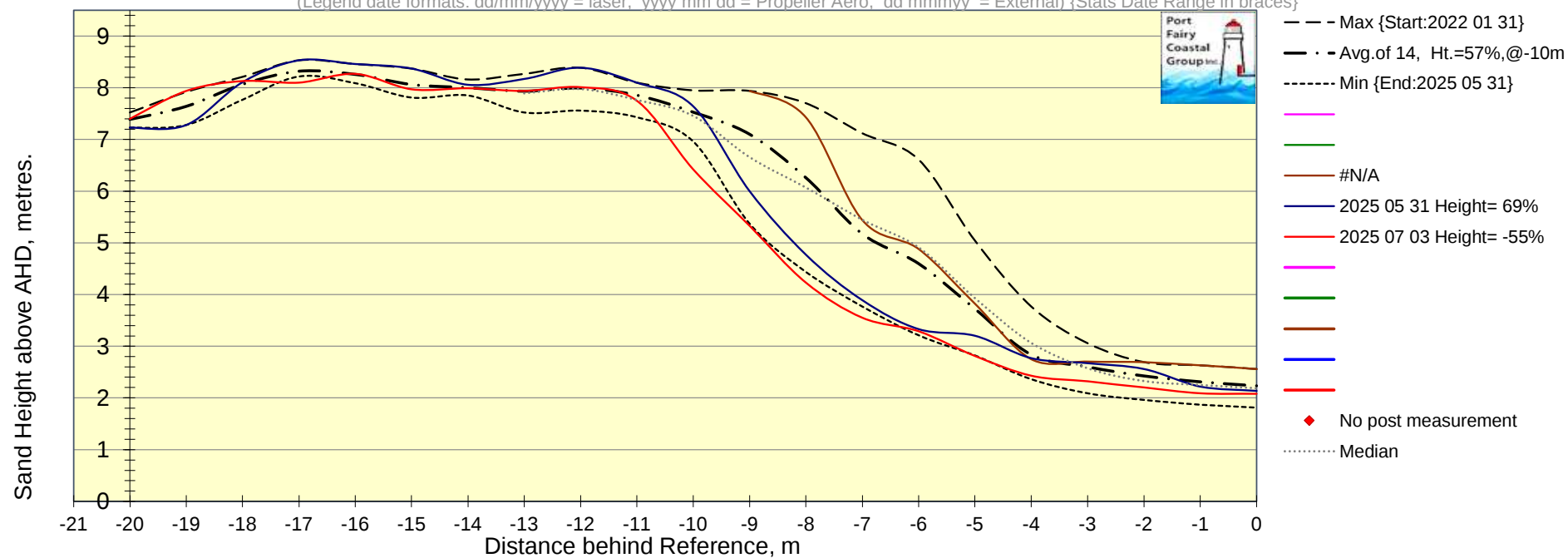
Chart PFETP10B Post 10B Transverse Profile of Dune Scarp.
