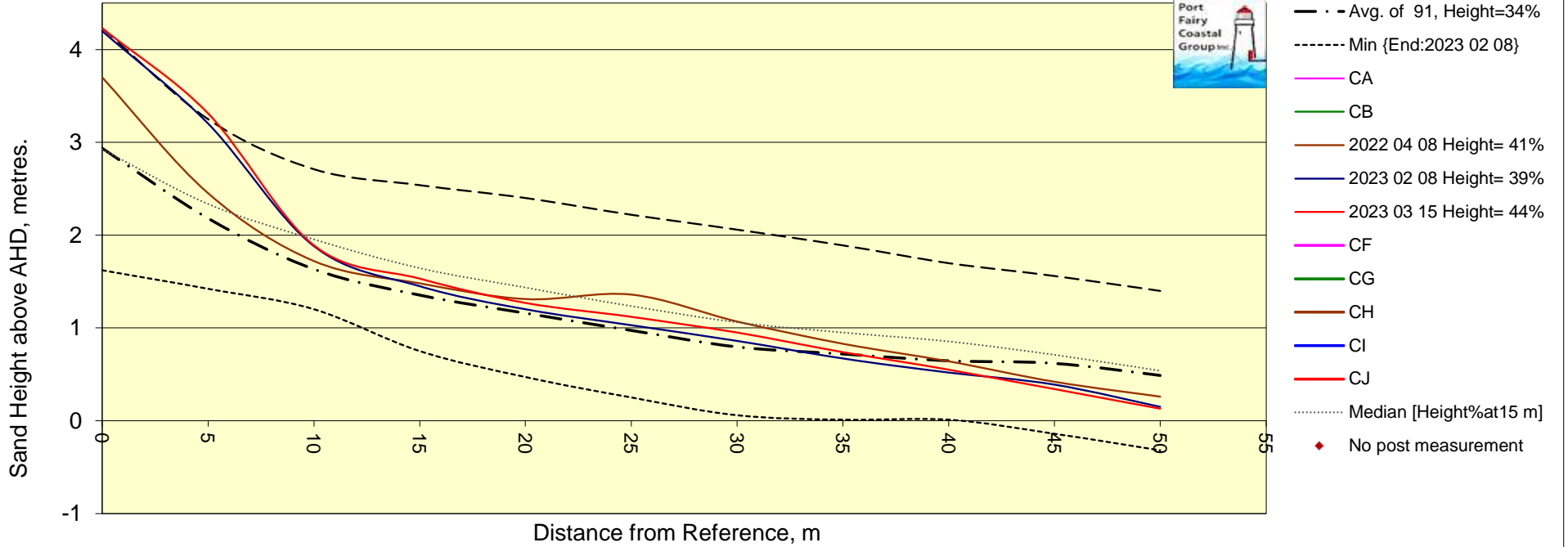
Chart PFETP4 Post 4 Transverse Profile perpendicular to dune scarp.
