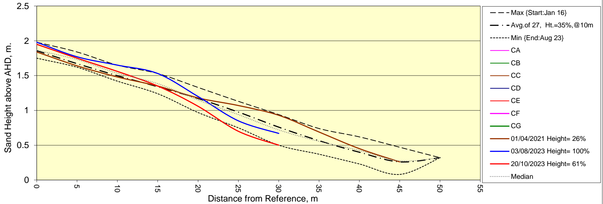
Chart PFSHTP21 Post 21, Transverse profile, Pea Soup 3. (Legend date formats: dd/mm/yyyy = laser, yyyy mm dd = Propeller Aero, yymmmdd = GPS)
