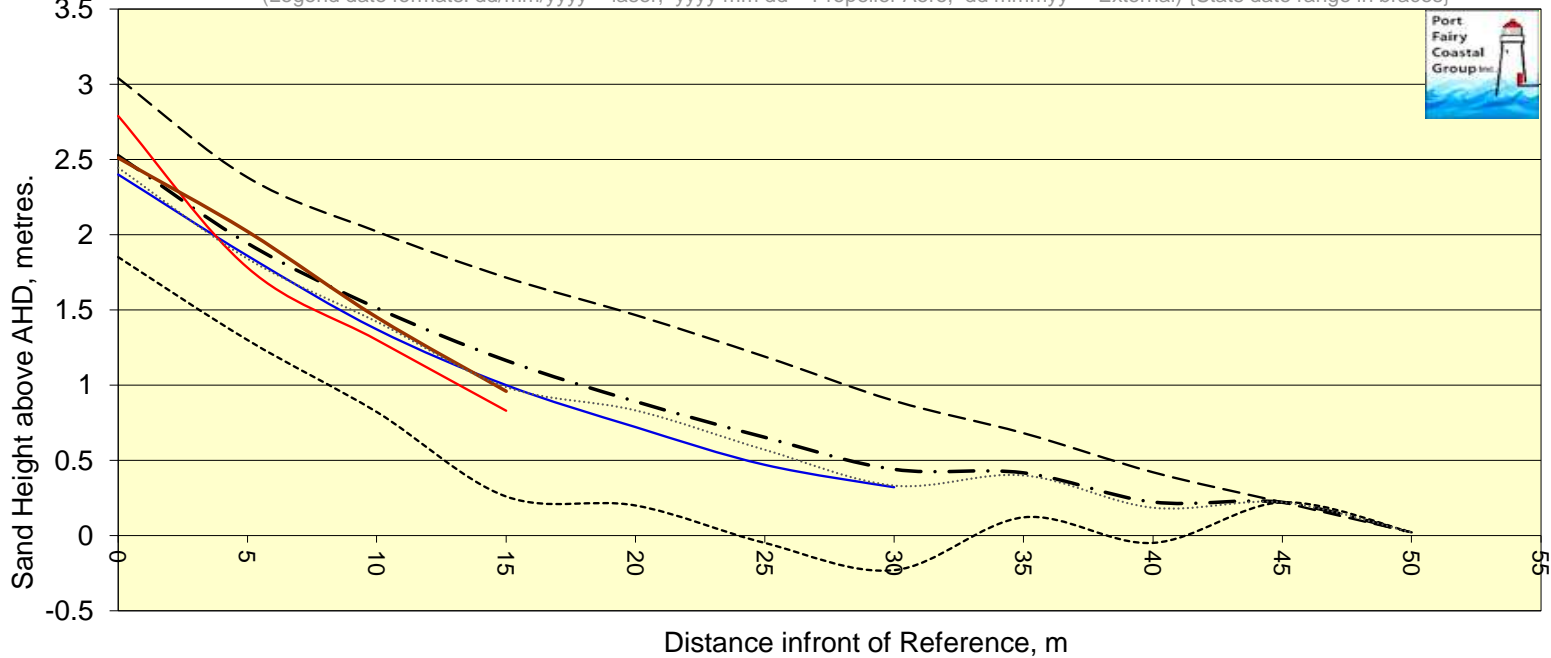
Chart PFETP10 Post 10 Transverse Profile perpendicular to dune scarp.
