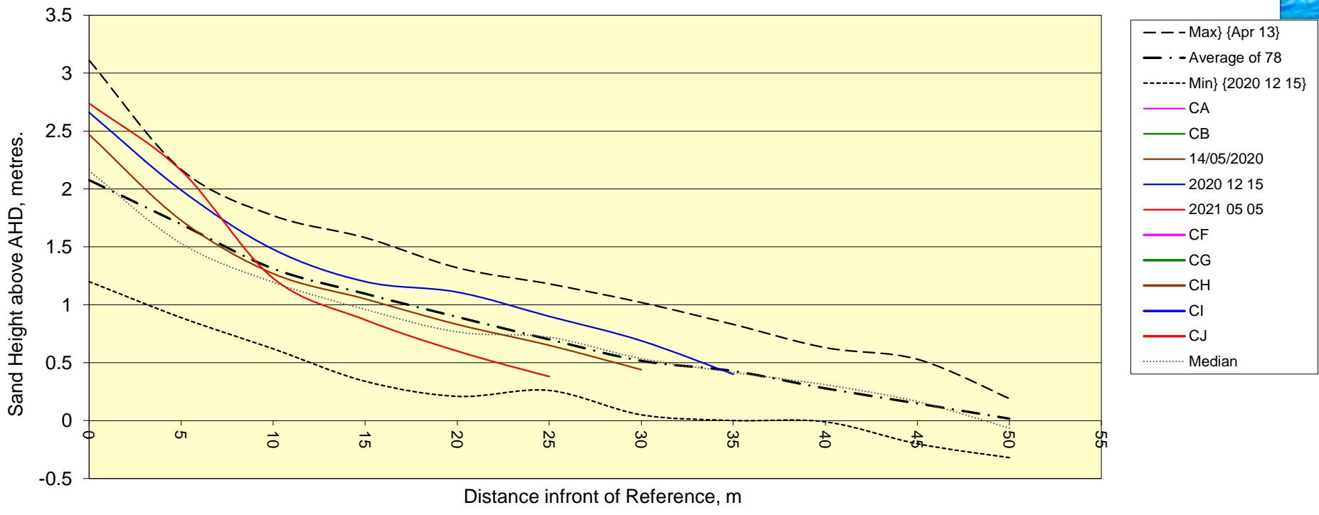
Chart PFEHTP8 Post 8 Transverse Profile perpendicular to dune scarp. (Legend date formats: dd/mm/yyyy = laser, yyyy mm dd = Propeller Aero, dd mmmmyy = GPS) {Stats date range in braces}
