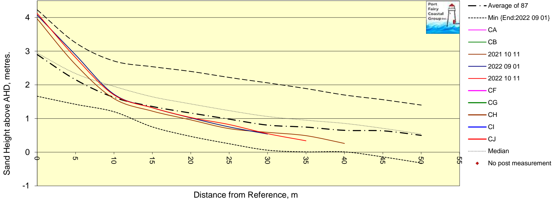
Chart PFETP4 Post 4 Transverse Profile perpendicular to dune scarp.
