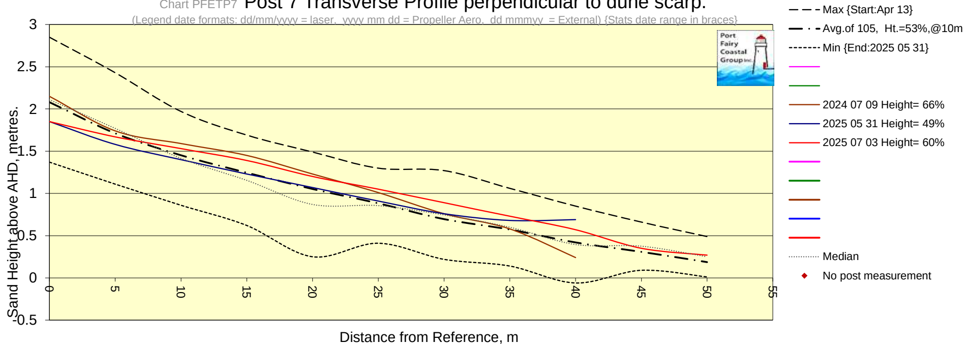
Chart PFETP7 Post 7 Transverse Profile perpendicular to dune scarp.
