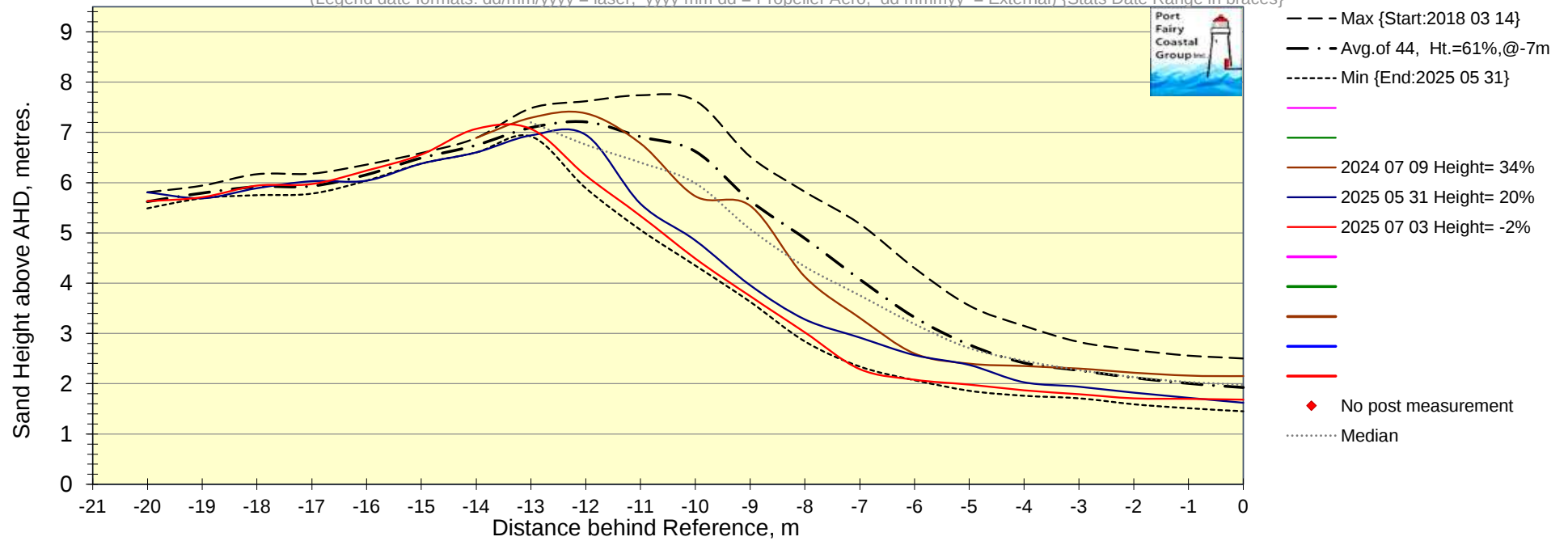
Chart PFETP9B Post 9B Transverse Profile of Dune Scarp.
