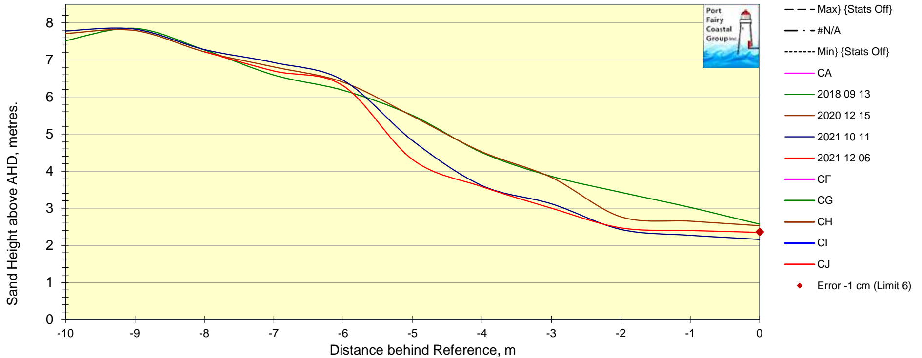
Chart PFETP10B Post 10B (Rear) Transverse Profile of Dune Scarp.
