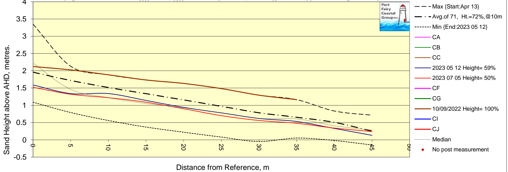
Chart PFETP1 Post 1 Transverse Profile perpendicular to dune scarp.
