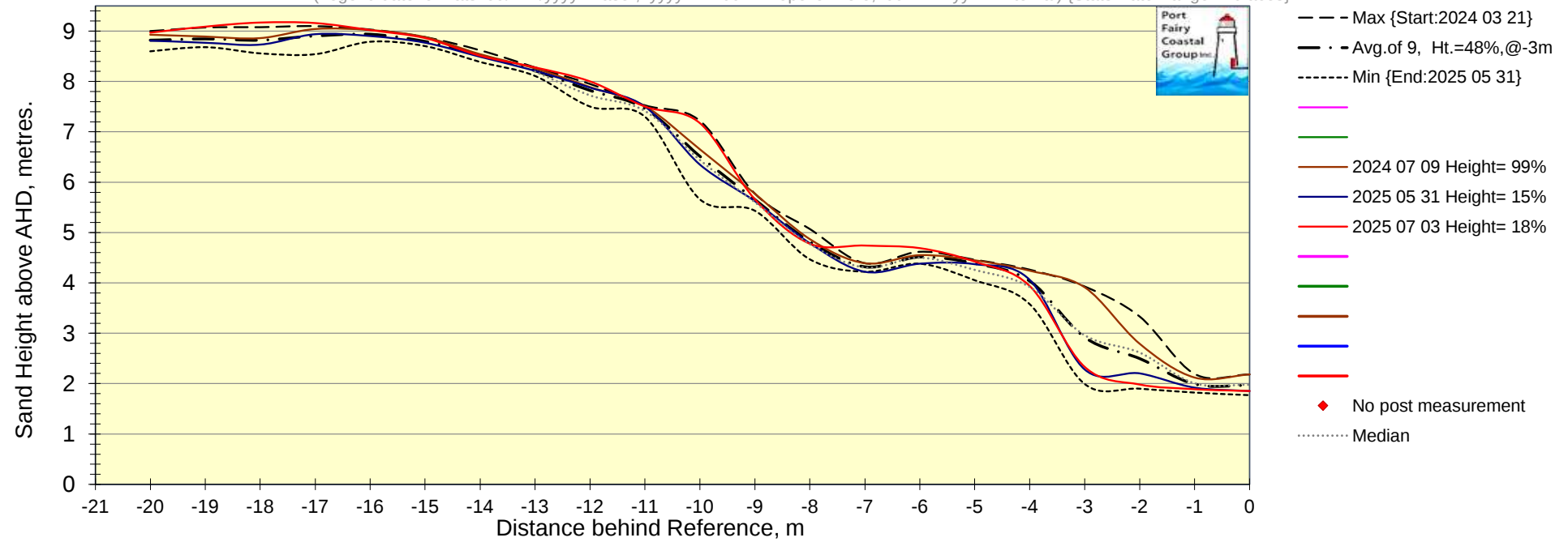
Chart PFETP9B Post 7B Transverse Profile of Dune Scarp.
