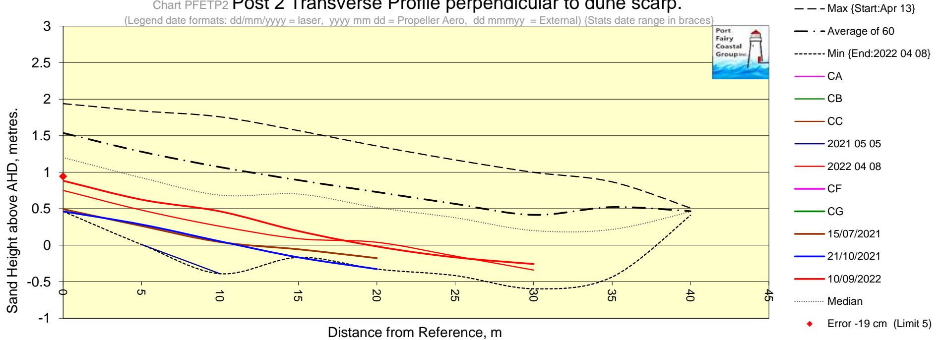
Chart PFETP2 Post 2 Transverse Profile perpendicular to dune scarp.
