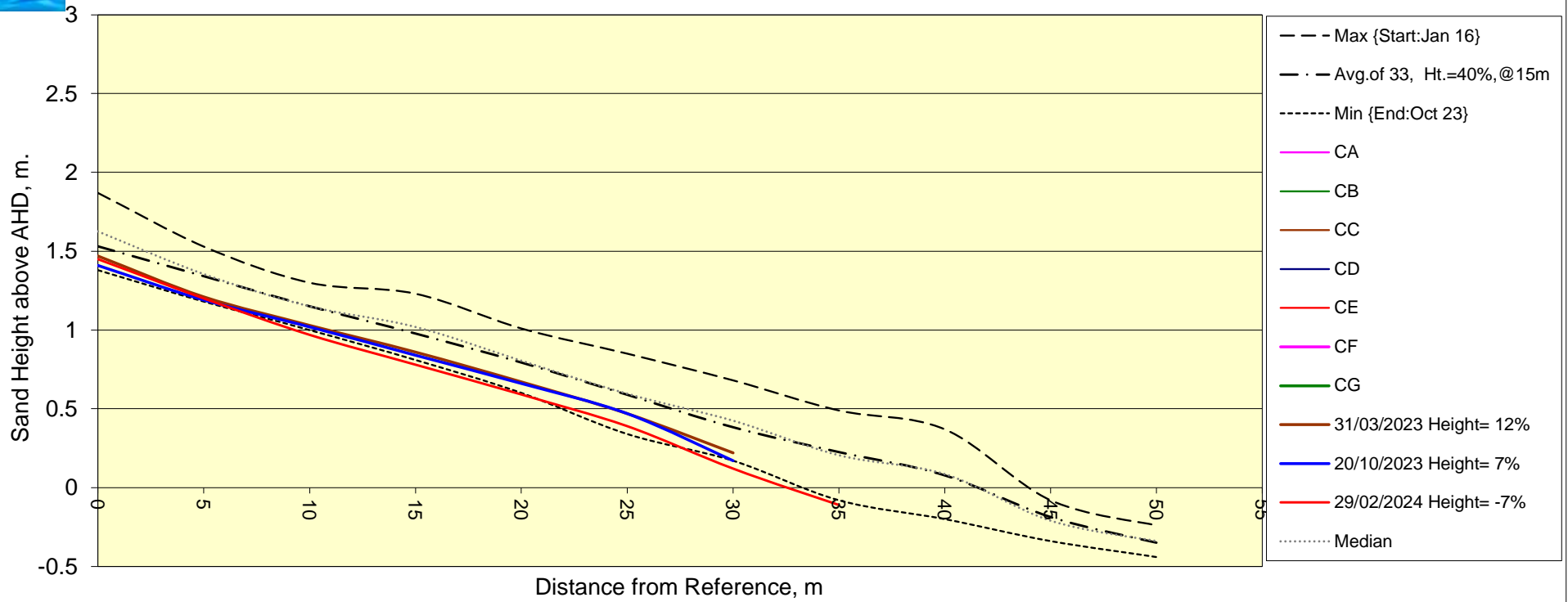
Chart PFSHTP22 Post 22 MSC117, Transverse profile, Pea Soup. (Legend date formats: dd/mm/yyyy = laser, yyyy mm dd = Propeller Aero, ddmmmyy = GPS, mmmyyyy = Other)
