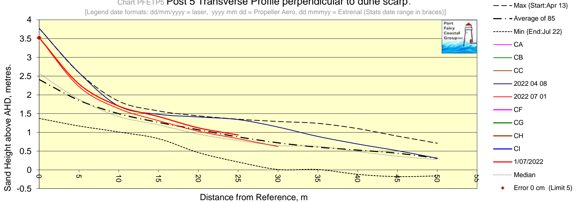
Chart PFETP5 Post 5 Transverse Profile perpendicular to dune scarp.
