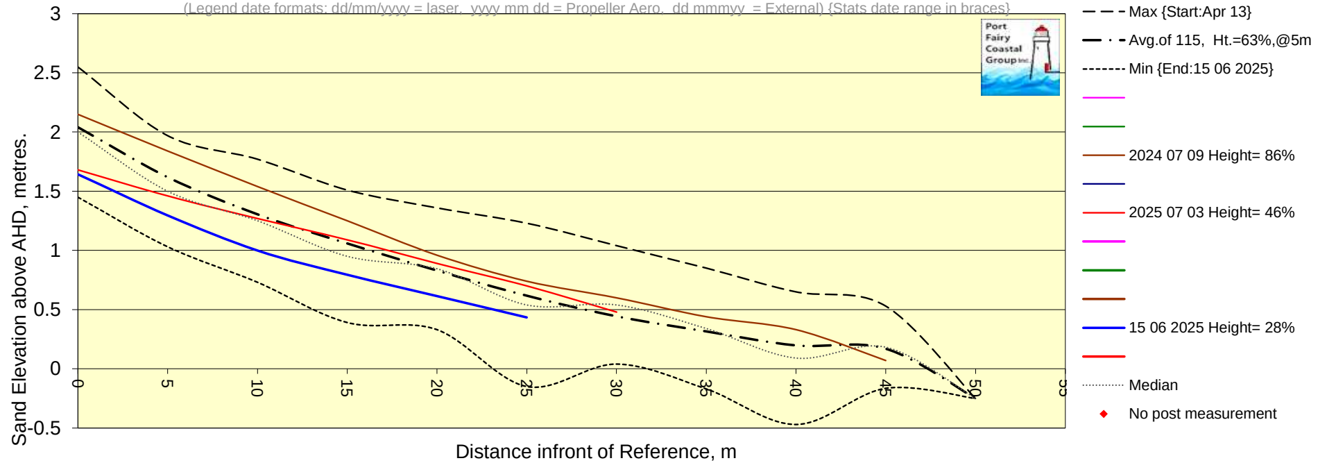
Chart PFETP9 Post 9 Transverse Profile perpendicular to dune scarp.
